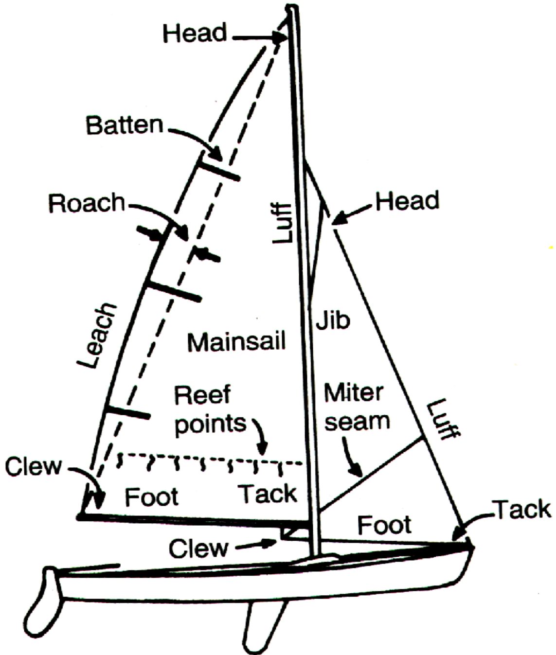
Sailboat Schematics with basic parts identified.
